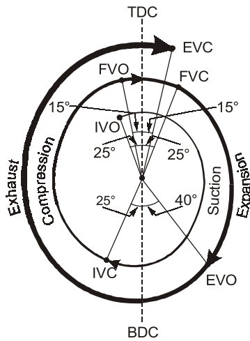
Fig. 1.16 : Valve Timing Diagram for a Four-Stroke Diesel Engine
