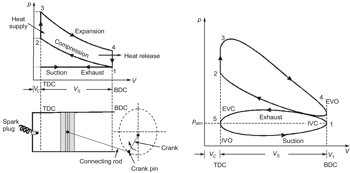
(a) Theoretical p-V diagram for a four-stroke petrol engine
